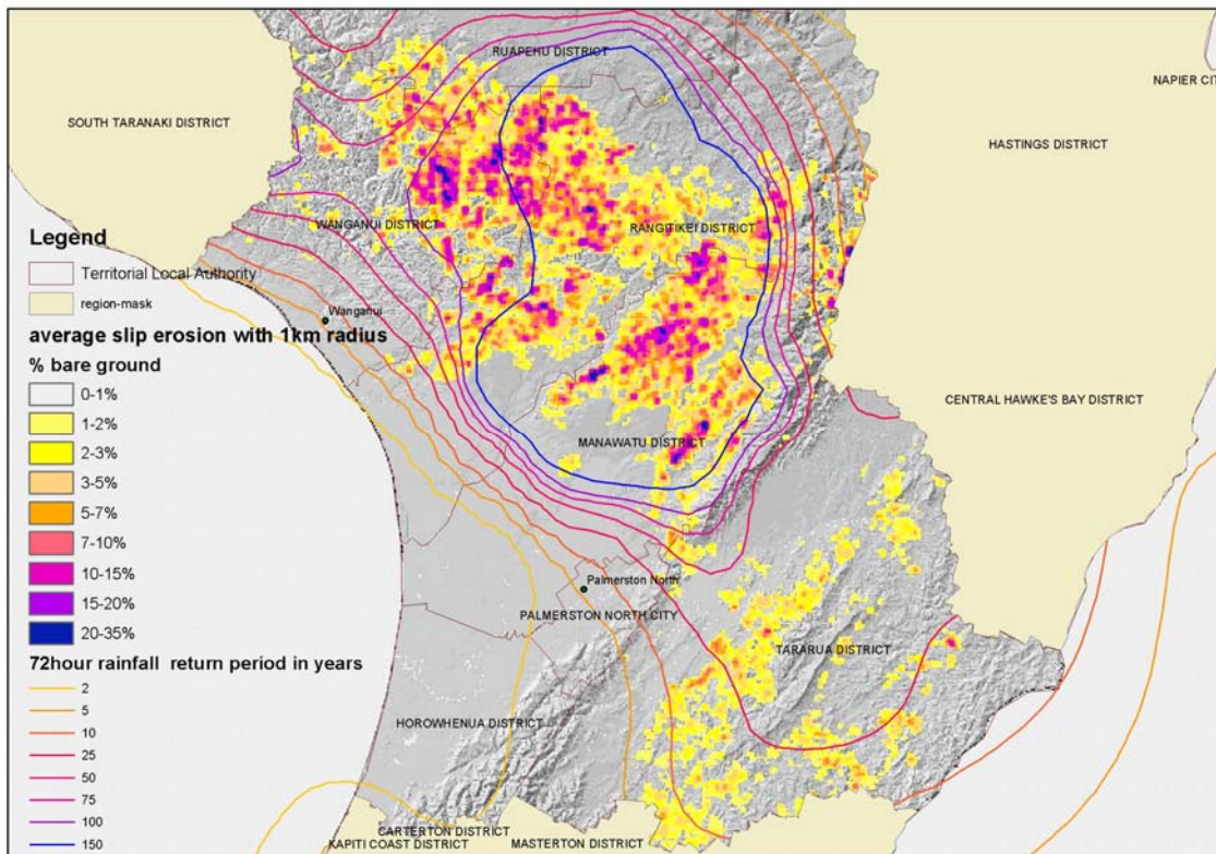
Figure 2: Rainfall return period isohyets (from NIWA) and severity of erosion (from Landcare Research) for the February storm
