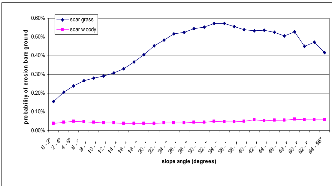
Figure 4: The effect of trees on landslide erosion (from Landcare Research)
