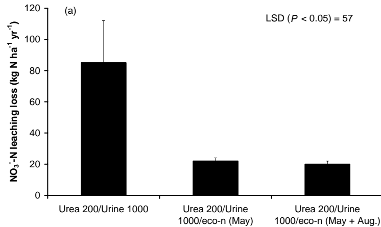
Figure 3. Total amount of nitrate leaching losses from large Templeton soil lysimeters following one application (May) and two applications (May and August) of eco-n (Di and Cameron, 2004b).
