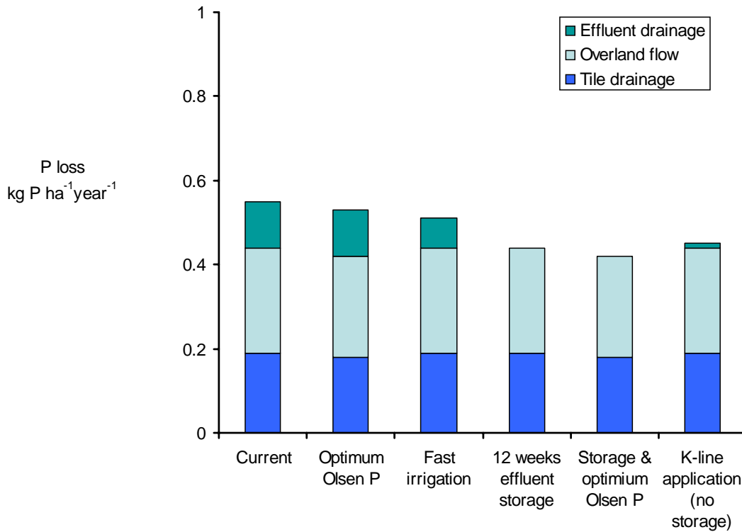
Figure 4. Modelled phosphorus (P) losses from farmland within the Bog Burn catchment under a range of BMP scenarios targeted at dairy farms only.
