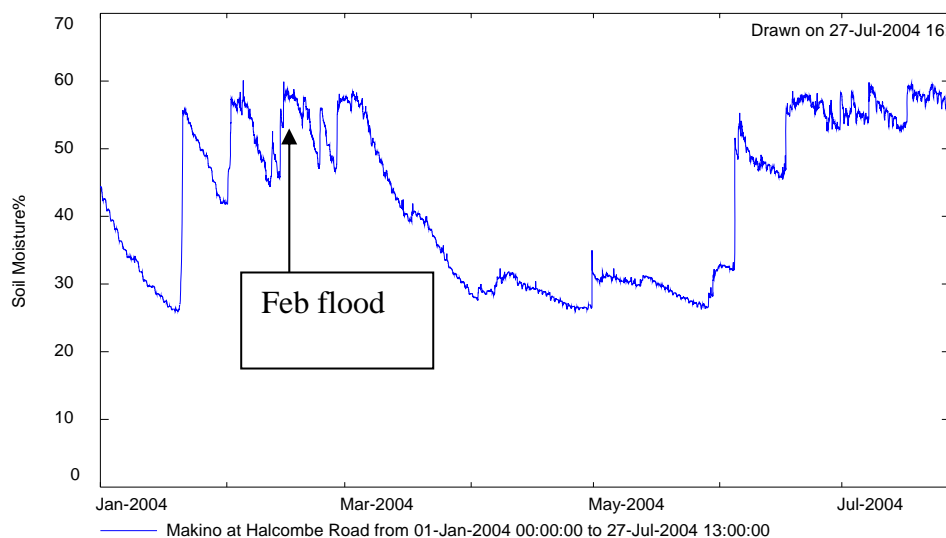
Figure 1: Soil moisture near Feilding
